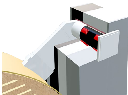
AIR CONTROL installation type LAL concealed within the reveal of round windows
