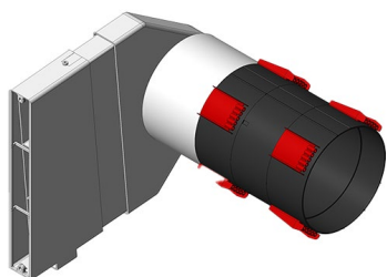
AIR CONTROL for short wall panes Installation in the reveal
